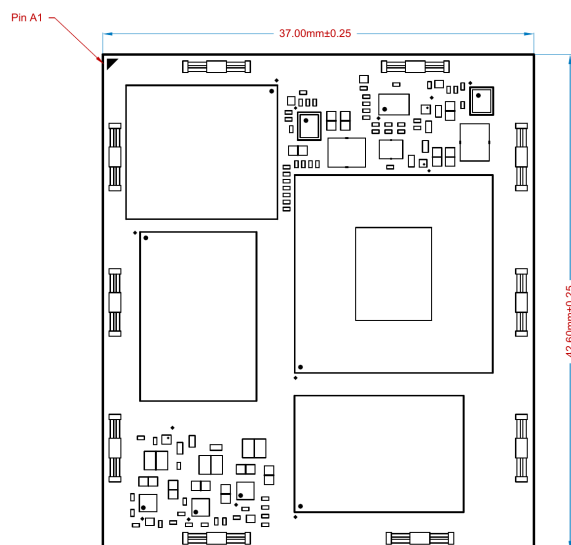
Figure 8: Grinn AstraSOM-1680 top view dimensions
