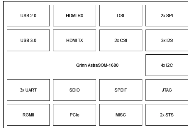
Figure 5: Grinn AstraSOM-1680 interfaces overview
