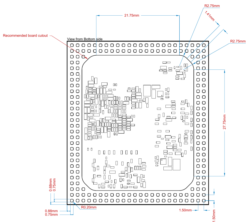
Figure 9: Grinn AstraSOM-1680 bottom view dimensions
