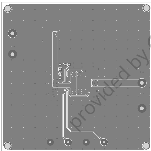
Figure 6: Mid-Layer 2
