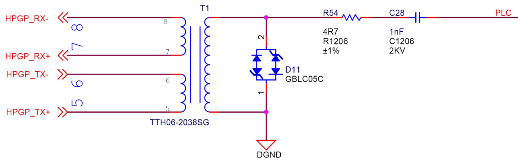
Figure 11 – HPGP Coupler Circuit
