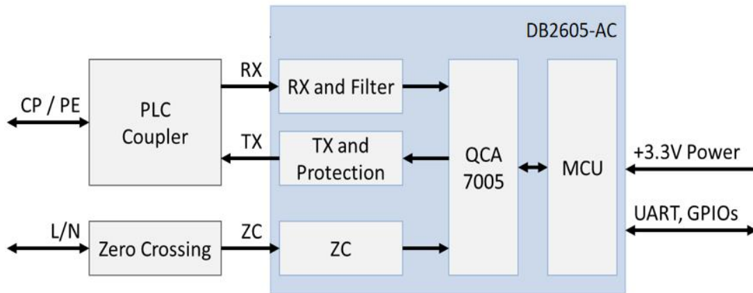
Figure 1 – DB2605-AC Block Diagram
