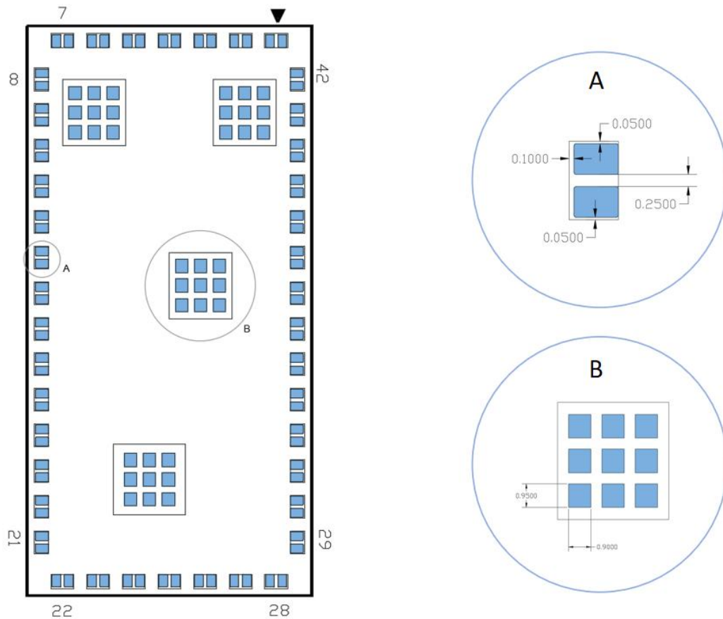
Figure 6 – Recommended Paste Footprint
