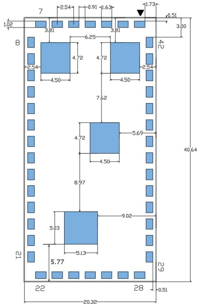
Figure 5 – Recommended Solder Footprint
