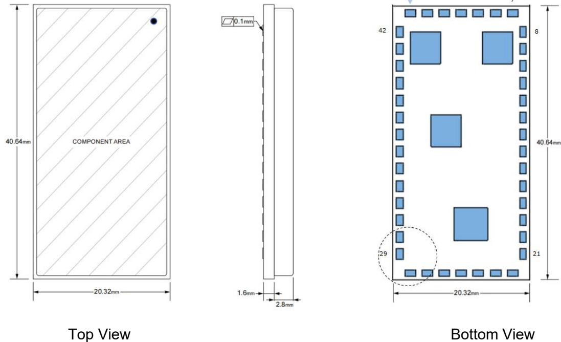
Figure 4 – DB2605-AC Form Factor
