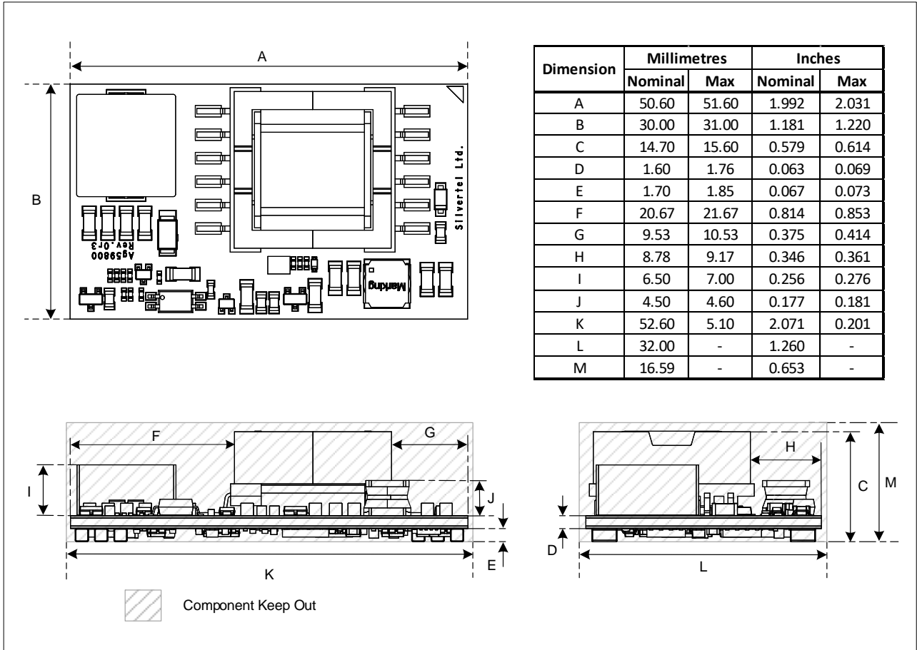
Figure 13: Package Dimensions
