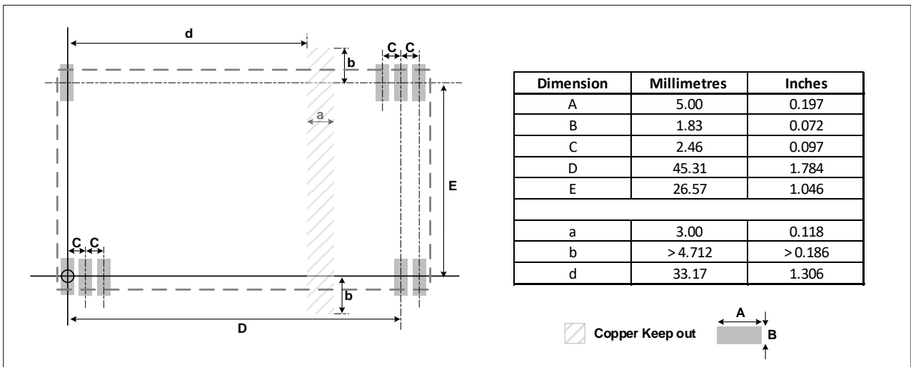
Figure 14: Land Pattern
